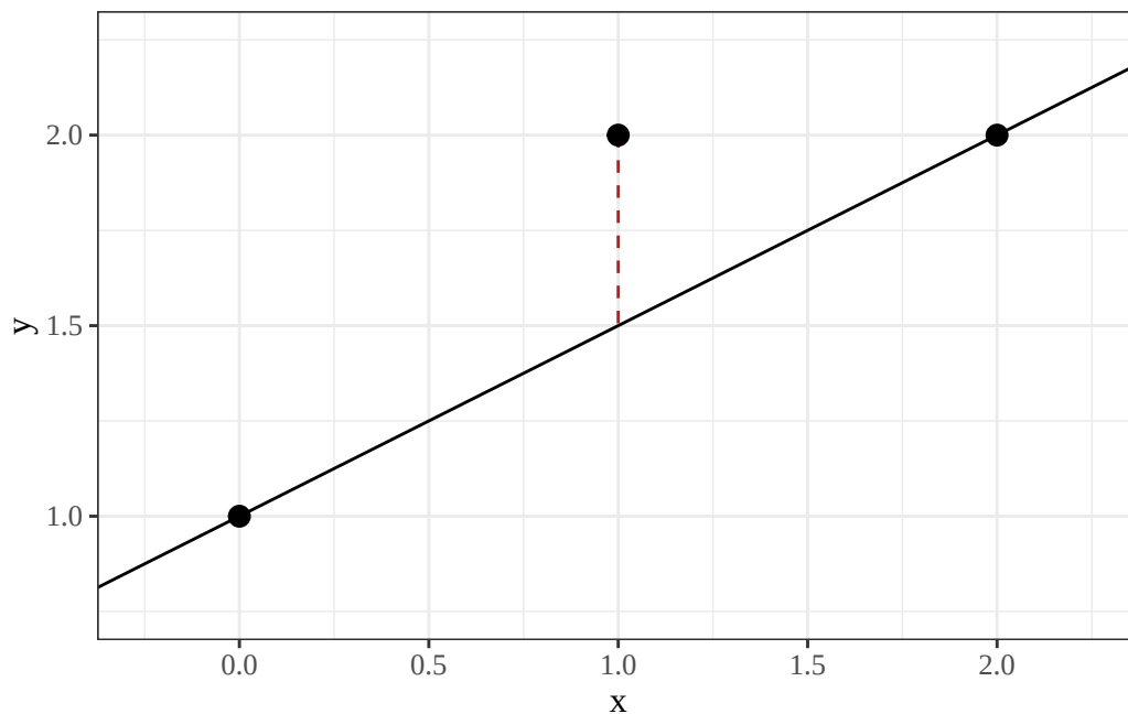
Figure 2: The three points, the line with intercept 1 and slope 0.5, and the one nonzero residual (dashed)
