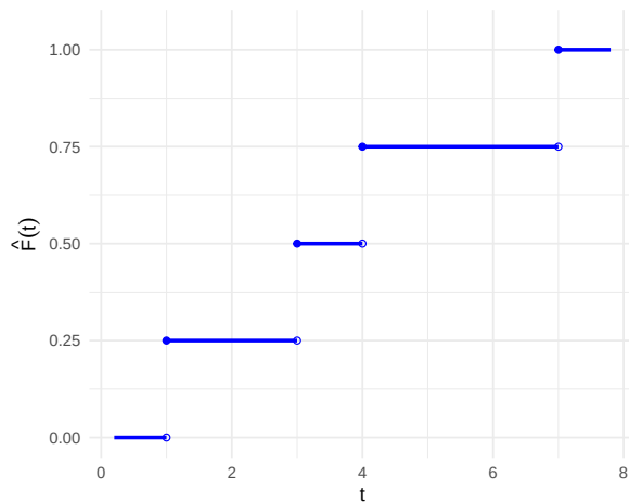
(a) Empirical CDF, horizontal pieces only. Closed circles mark included endpoints; open circles mark excluded endpoints.
