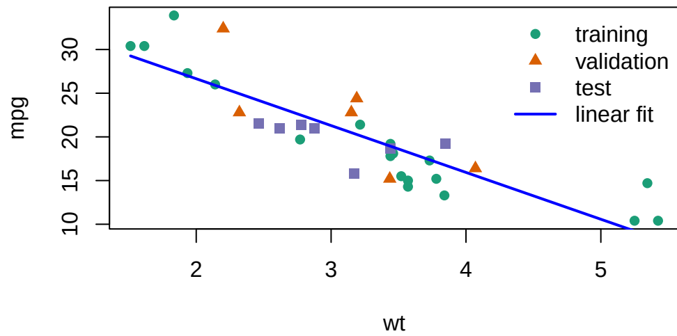
Figure 2: Linear model fit superimposed on data partitions
