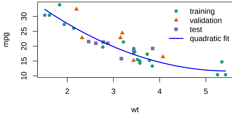
Figure 3: Quadratic model fit superimposed on data partitions
