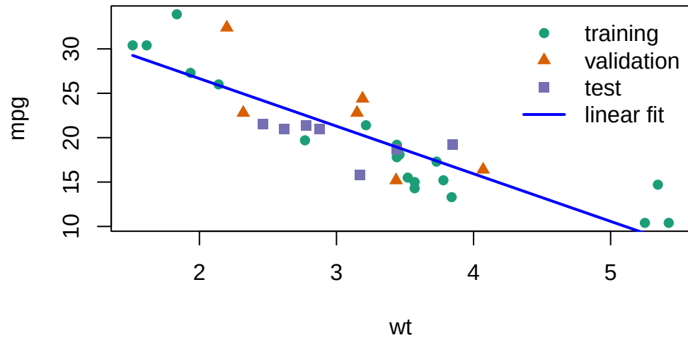
Figure 2: Linear model fit superimposed on data partitions
