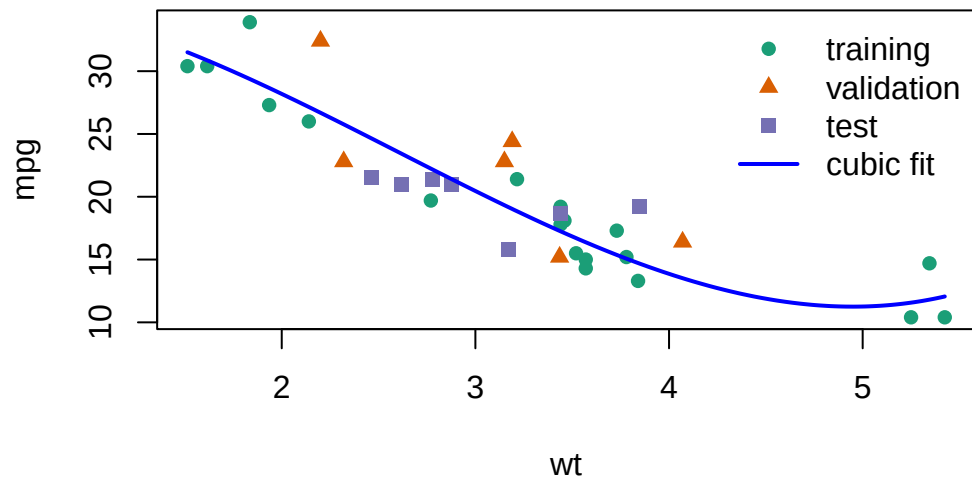
Figure 4: Cubic model fit superimposed on data partitions
