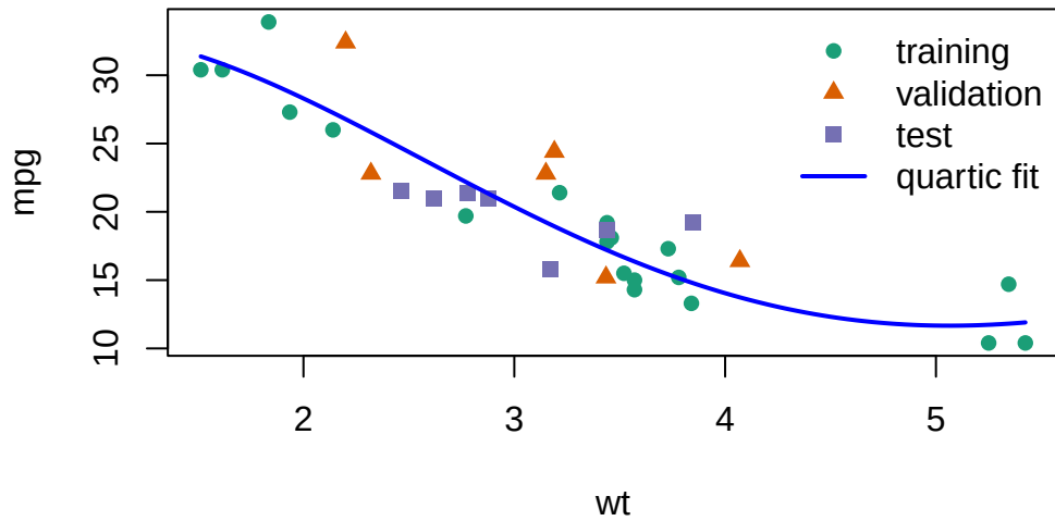
Figure 5: Quartic model fit superimposed on data partitions
