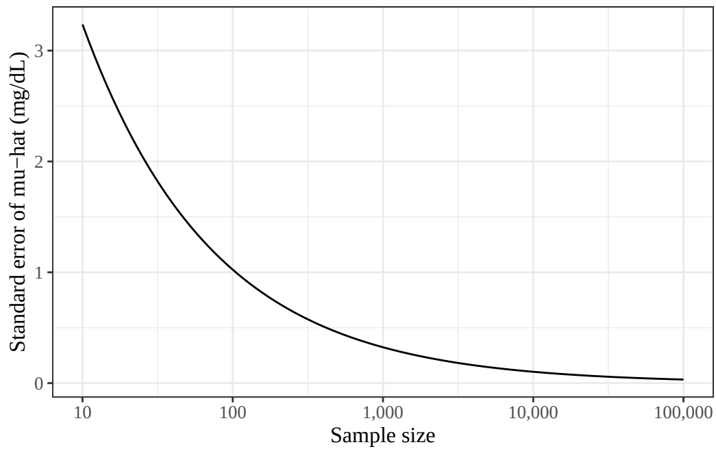
Figure 19: Standard error of \hat{\mu}_{\text{ML}} as a function of sample size, with \sigma = \hat{\sigma}_{\text{ML}}
