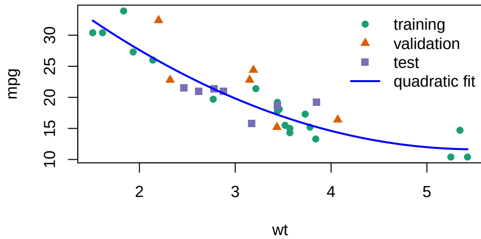
Figure 3: Quadratic model fit superimposed on data partitions
