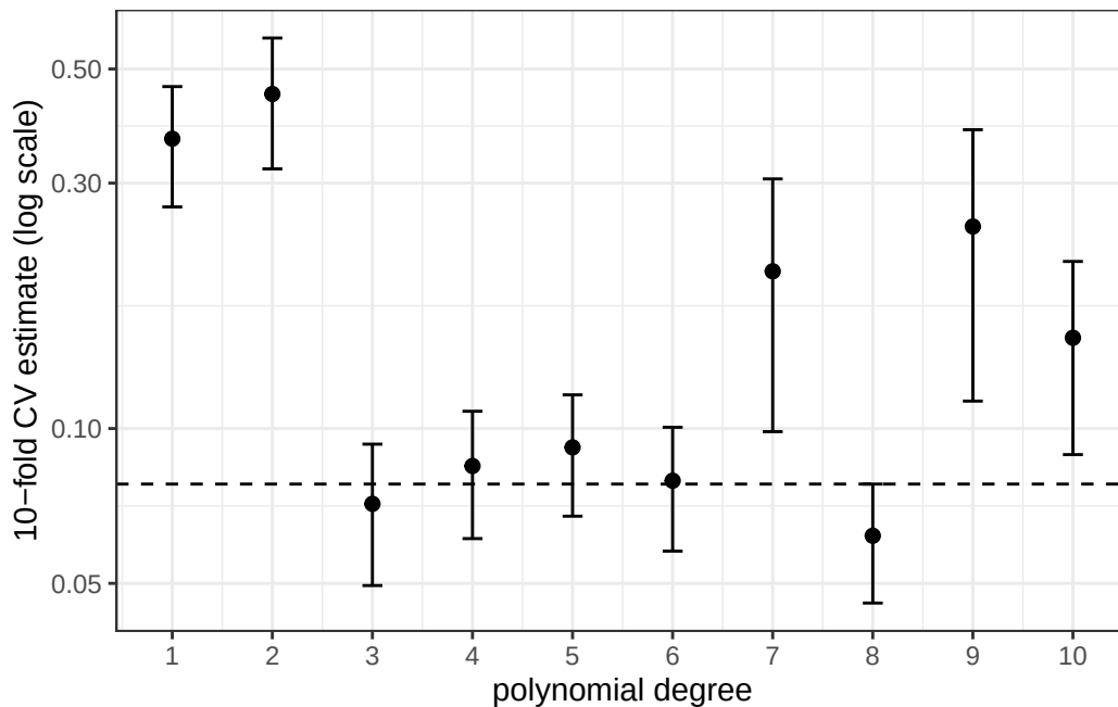
Figure 7: 10-fold cross-validation estimates, with bars of one fold-based standard error (Equation 35). The dashed line is one fold-based standard error above the smallest estimate.
