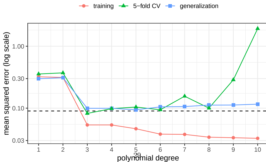
Figure 6: Figure 1 with the 5-fold cross-validation estimate added. Only the training and cross-validation curves could be computed from real data.
