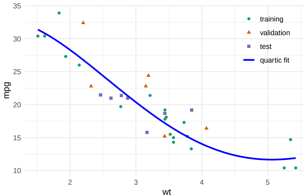
Figure 5: Quartic model fit superimposed on data partitions
