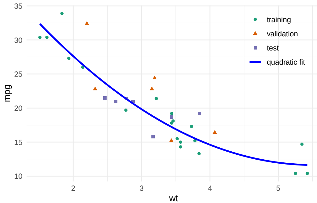
Figure 3: Quadratic model fit superimposed on data partitions
