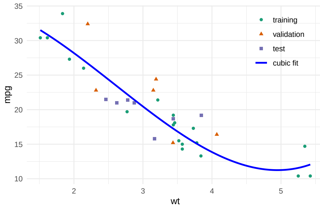
Figure 4: Cubic model fit superimposed on data partitions
