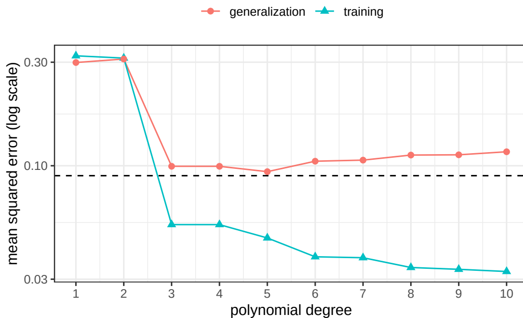
Figure 1: Training mean squared error and estimated generalization error (mean squared error on 10,000 new observations) of polynomial fits to one simulated training set of n = 30 . The dashed line is the noise variance \sigma^2 , the irreducible error .
