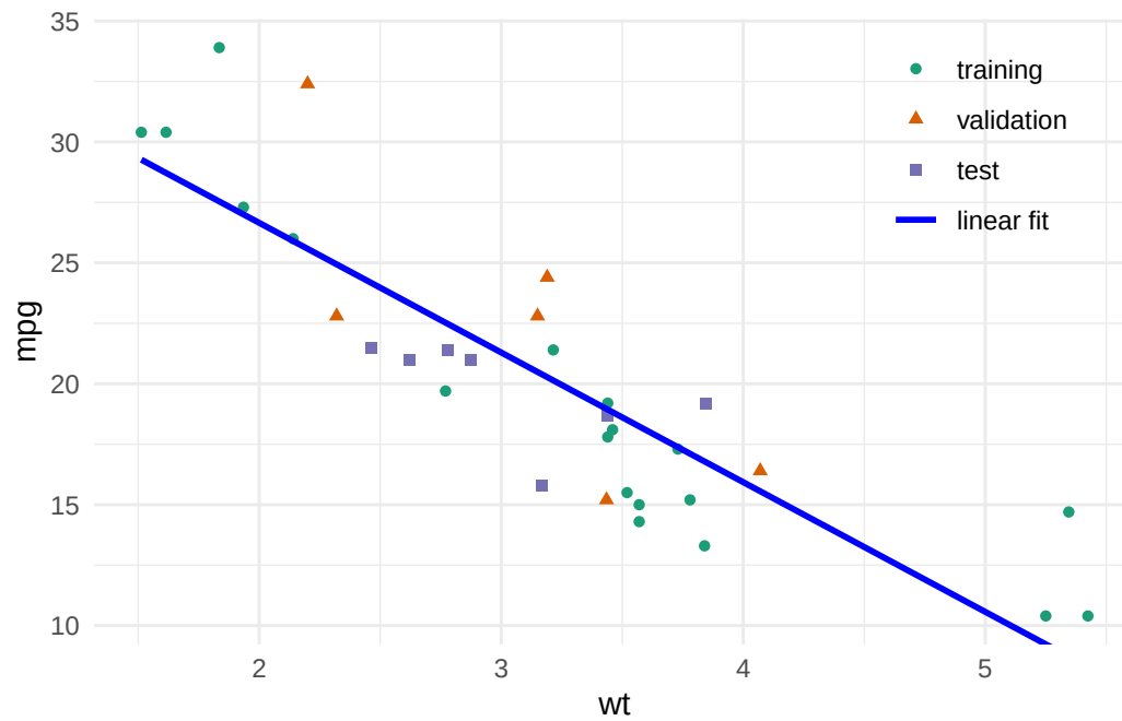
Figure 2: Linear model fit superimposed on data partitions
