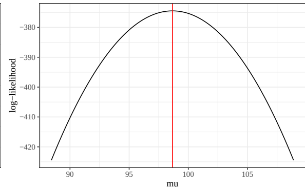
(b) Log-likelihood
