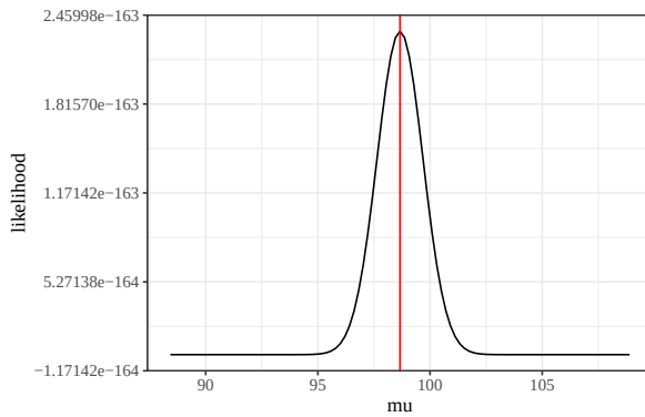
(a) Likelihood
