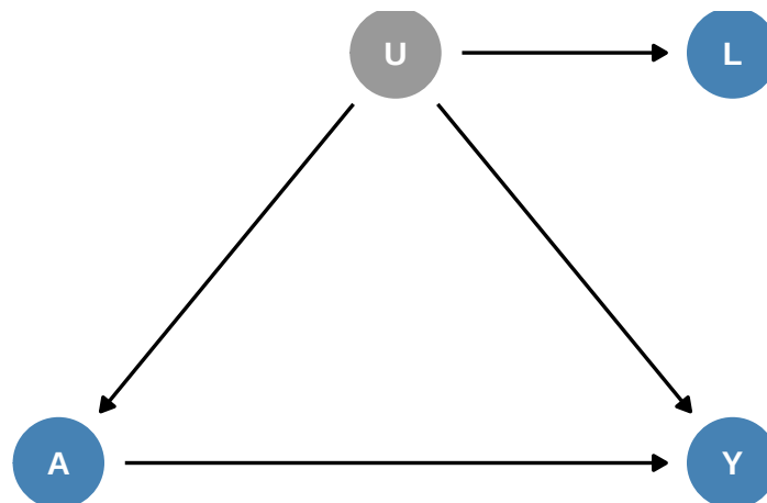
Figure 4: Figure 7.8. L is a surrogate (proxy) for the unmeasured common cause U of A and Y .
