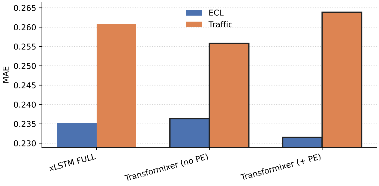
Controlled mixer ablation (MAE), lookback/horizon = 96 (y-axis zoomed; NLinear-only omitted for scale)
