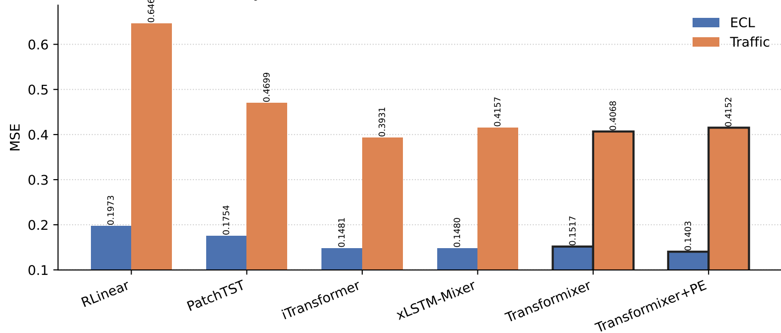
Long-term forecasting (MSE), lookback/horizon = 96 (y-axis zoomed; Informer omitted for scale)
