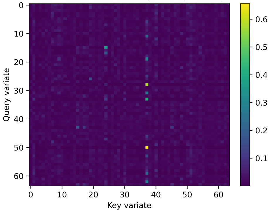
Transformixer attention (head 0, subset)
