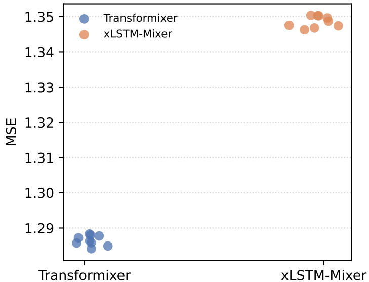
MSE under random channel permutations
