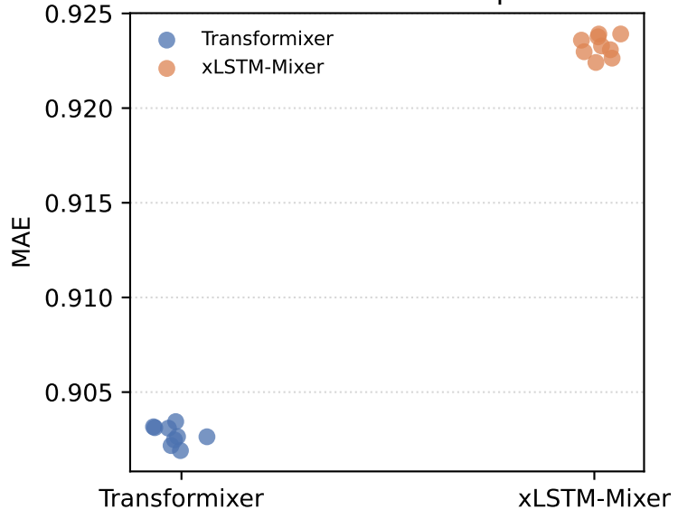
MAE under random channel permutations
