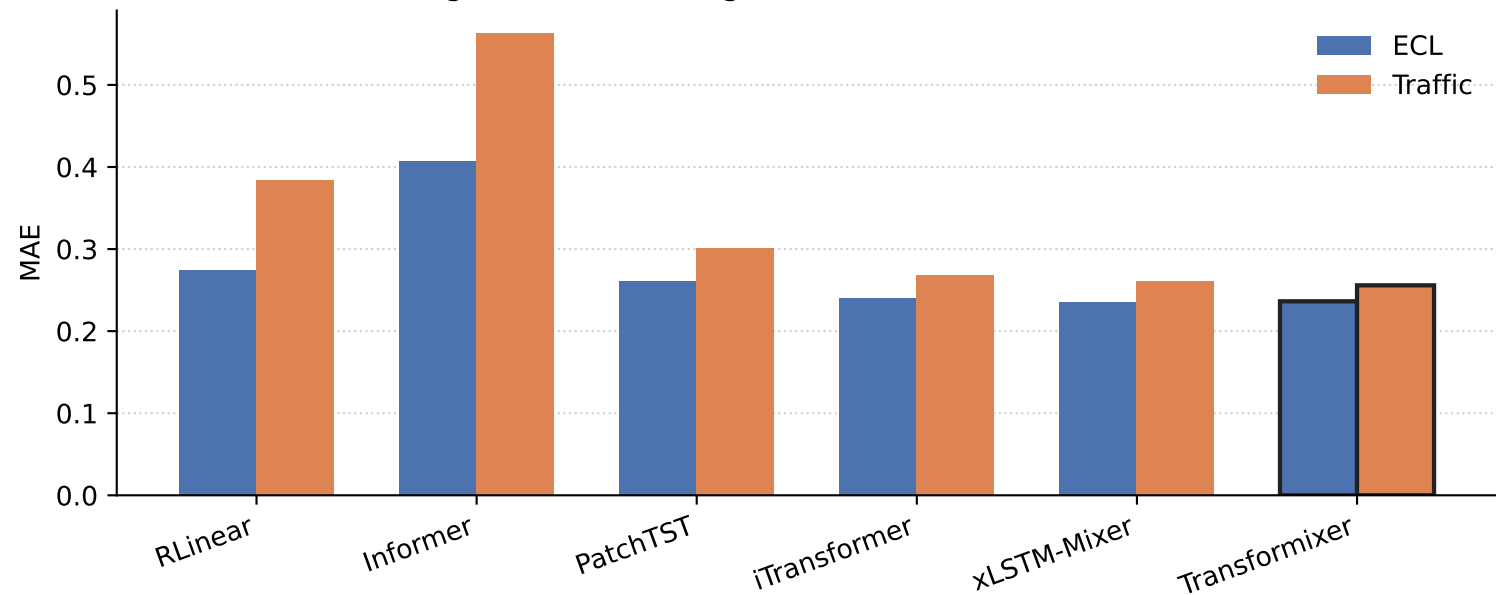
Long-term forecasting (MAE), lookback/horizon = 96
