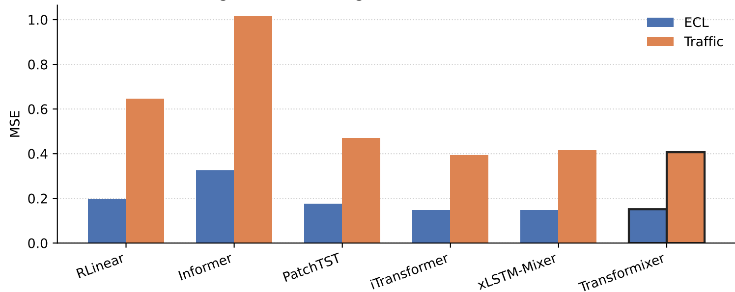
Long-term forecasting (MSE), lookback/horizon = 96
