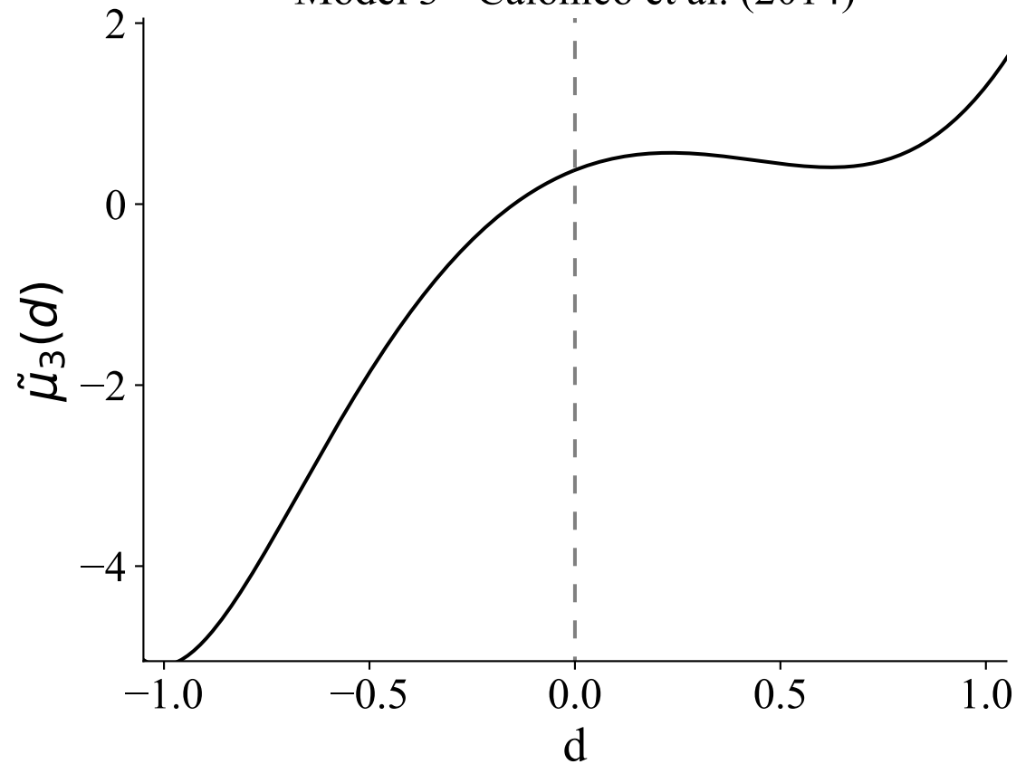
Model 3 - Calonico et al. (2014)
