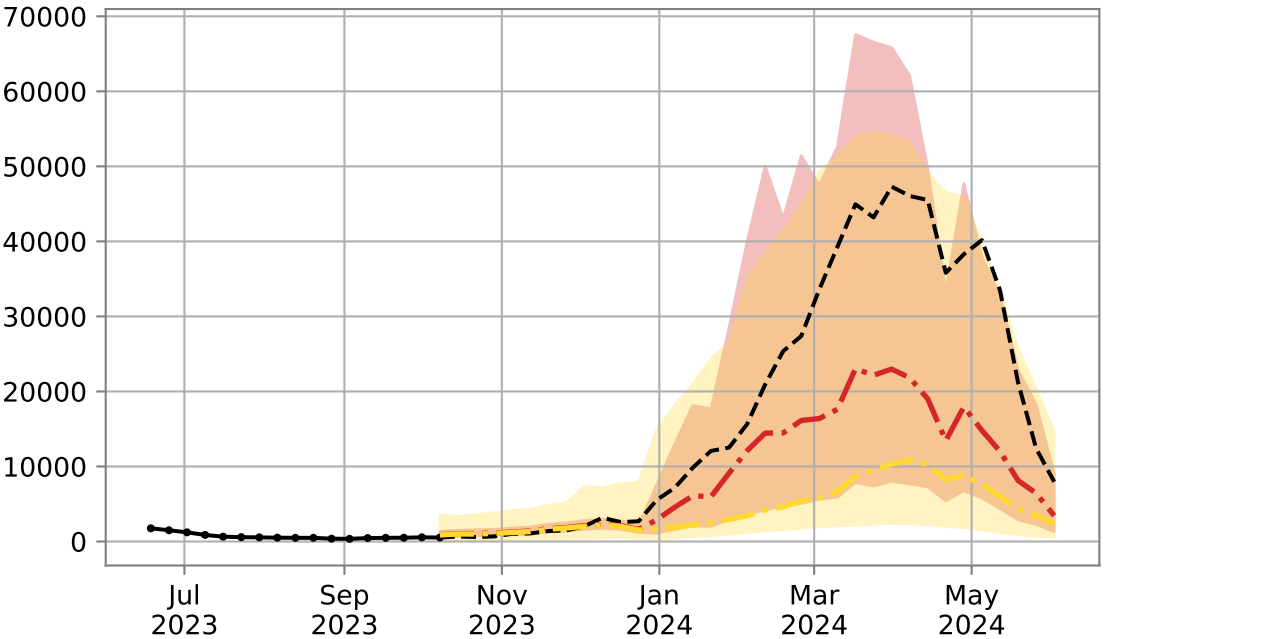
Forecast - PR - 2024
