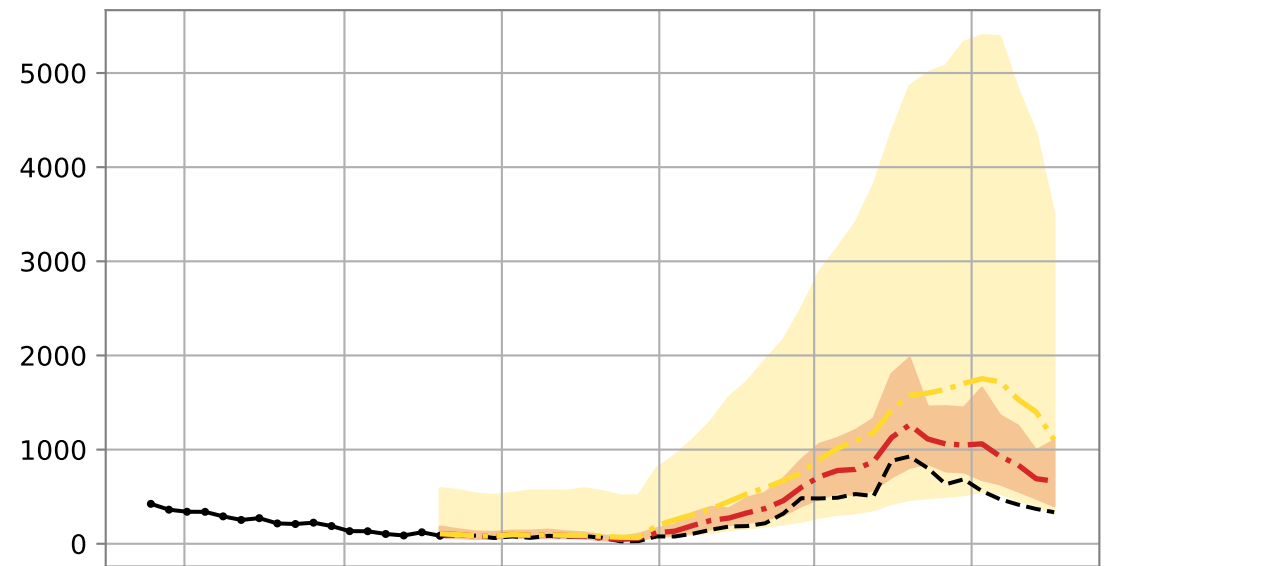
Forecast - GO - 2024
