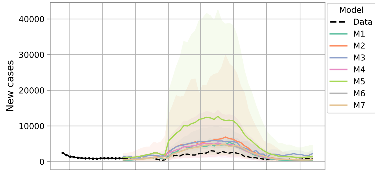
Forecast - GO - 2024
