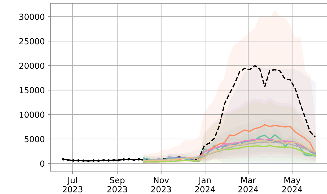
Forecast - GO - 2024
