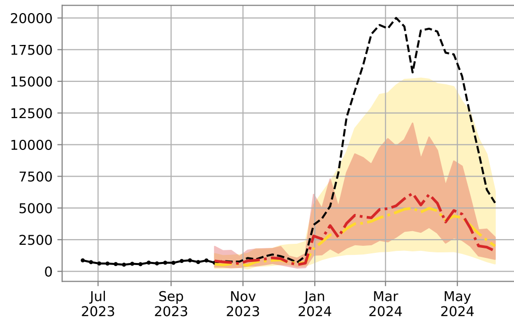
Forecast - GO - 2024
