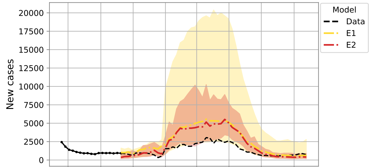
Forecast - GO - 2024
