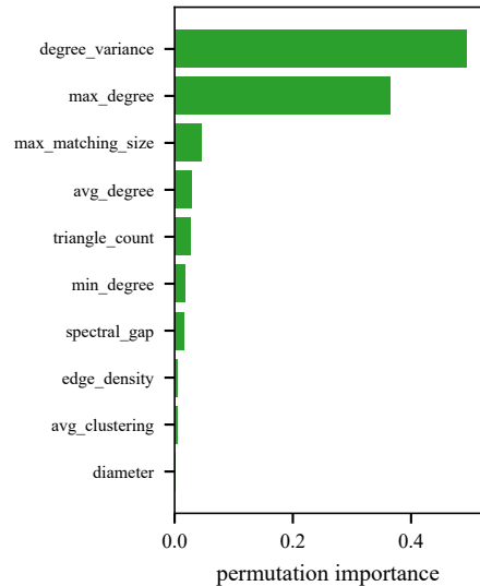
hybrid
