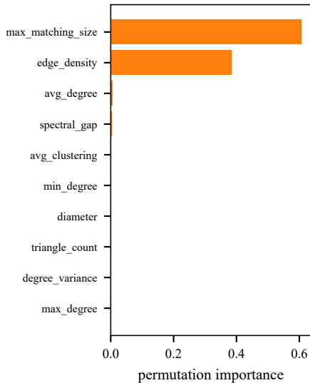
structured
