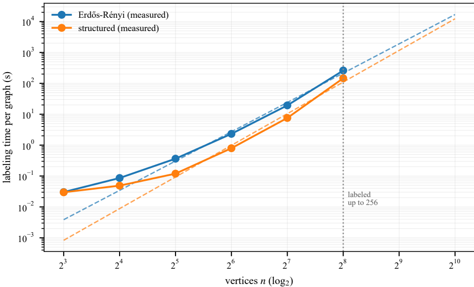
Measured labeling cost, with power-law extrapolation
