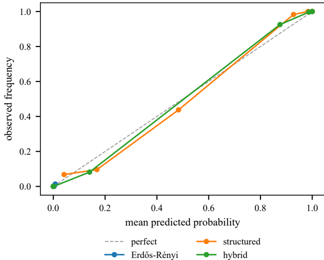
Calibration (reliability)
