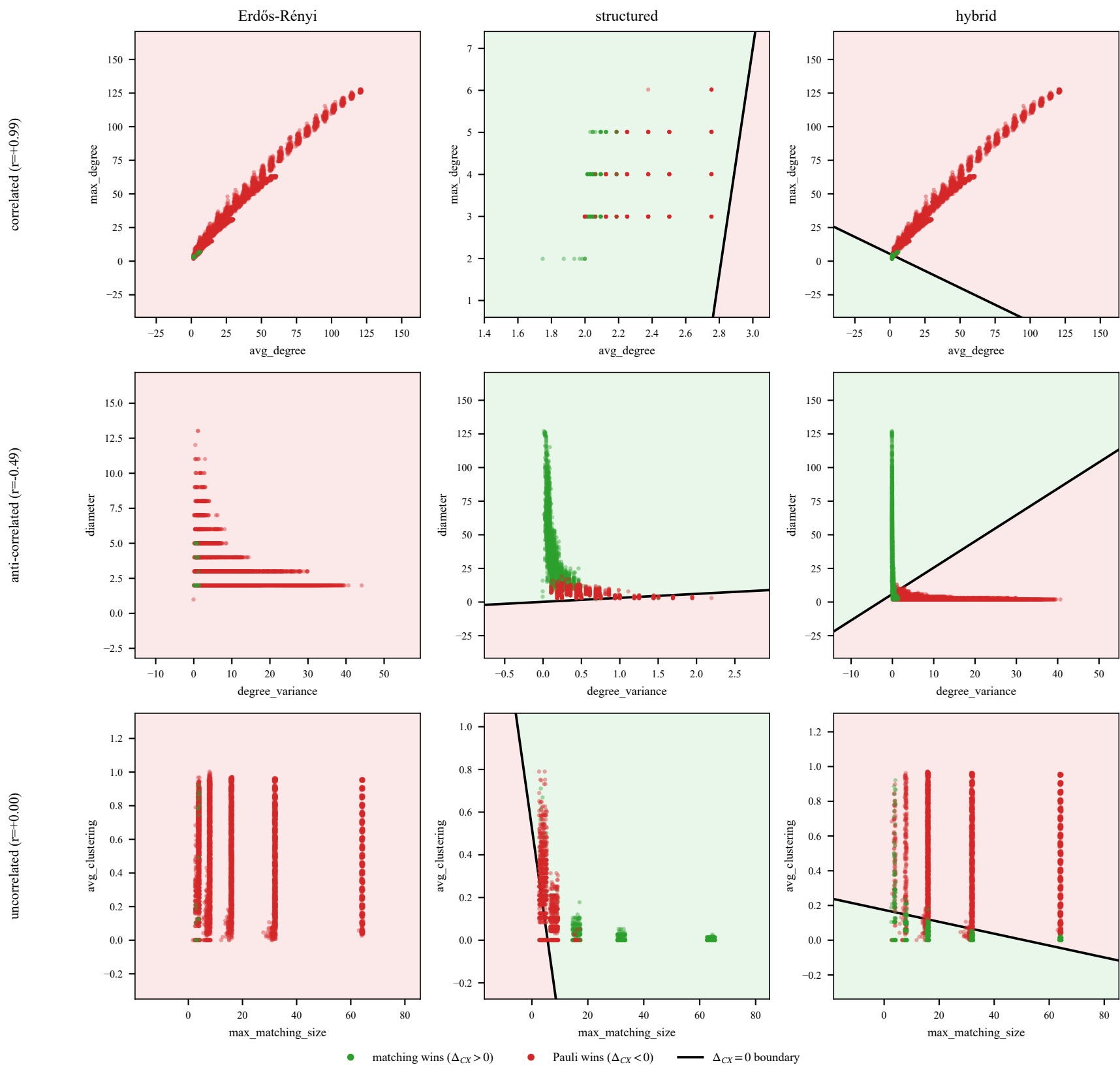
Trained logistic model's decision boundary, projected onto the best-separating pair per correlation band (others at median)
