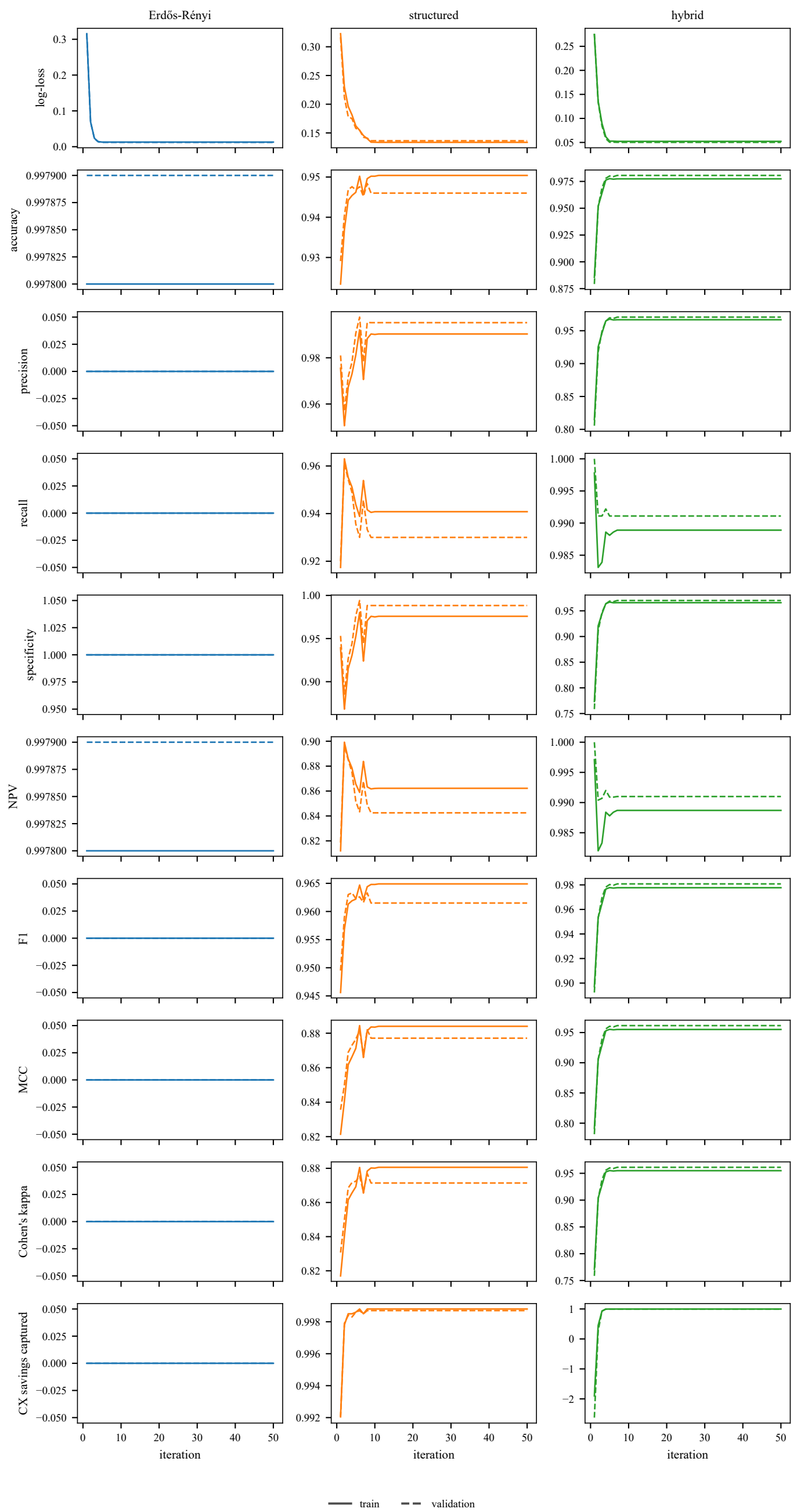
Logistic regression: training vs validation
