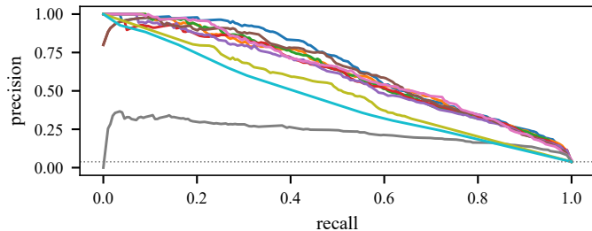
Precision-Recall
