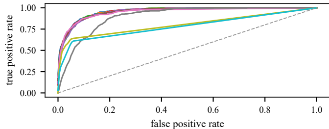
ROC curve
