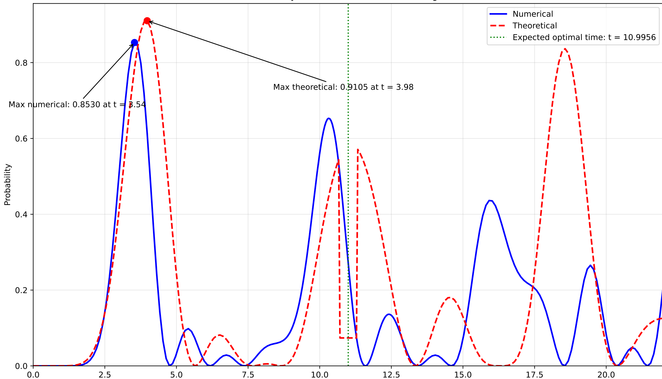
Exit Probability for BWT Quantum Walk (height = 3)
