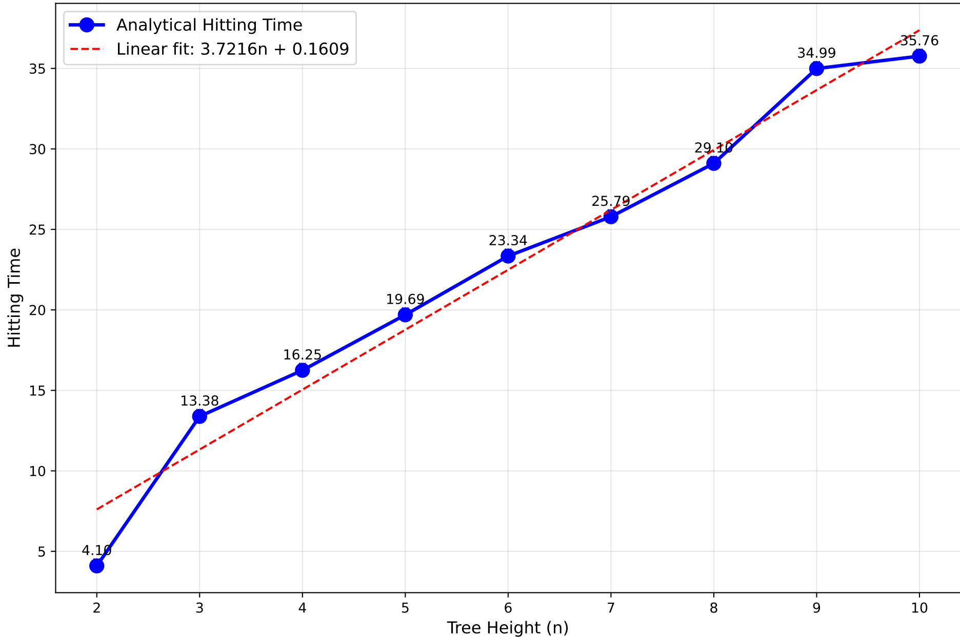
Analytical Hitting Time vs. BWT Height
