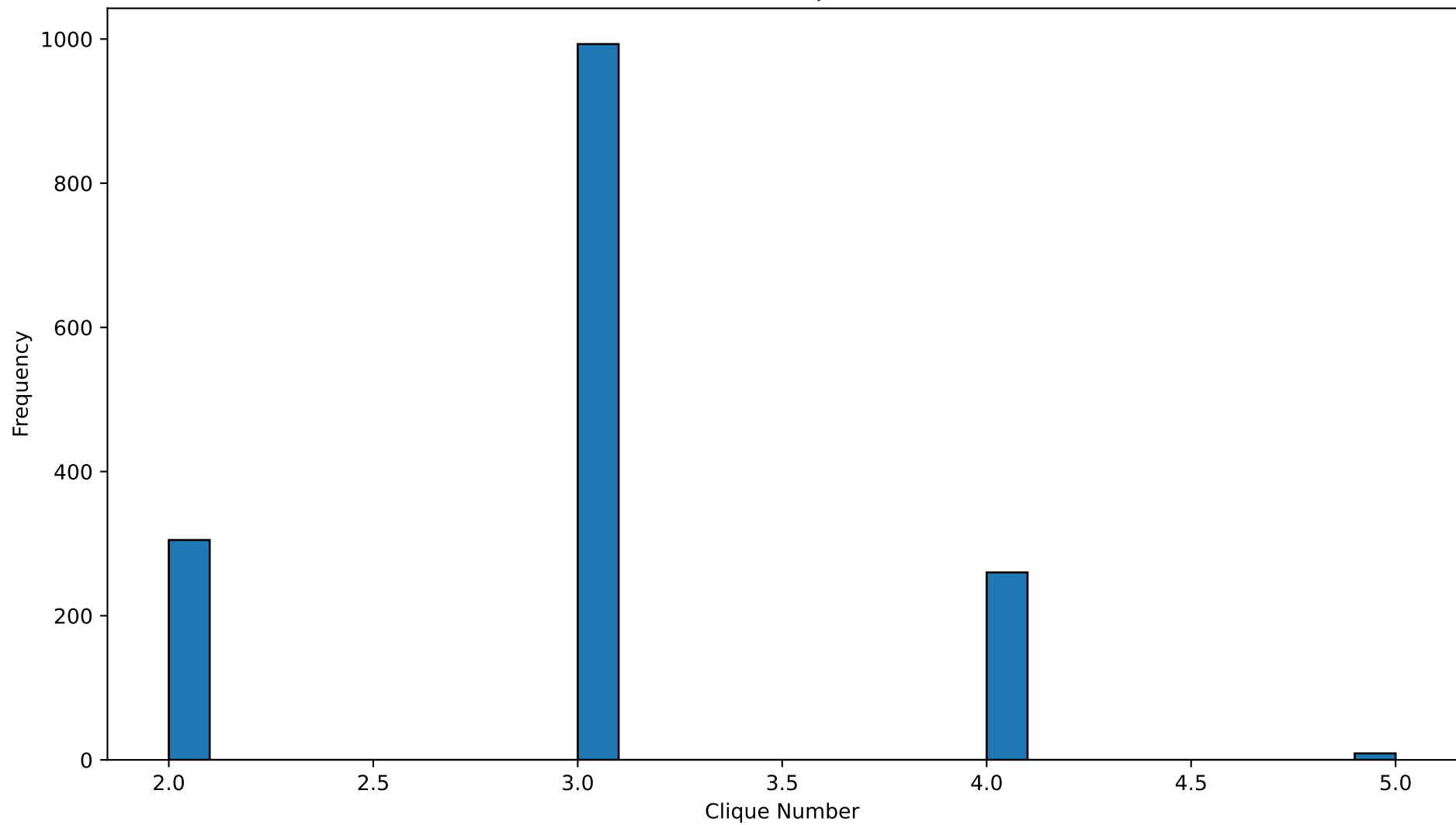
Distribution of Clique Numbers
