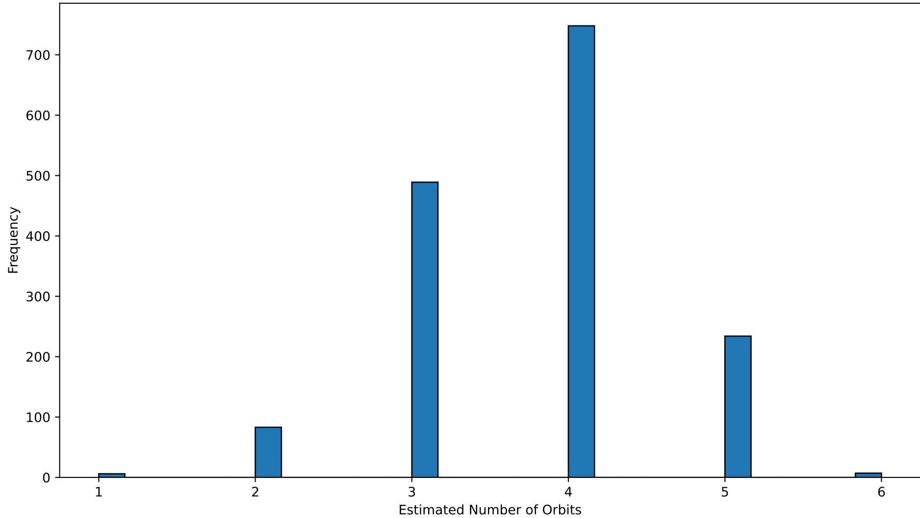
Distribution of Estimated Orbit Counts
