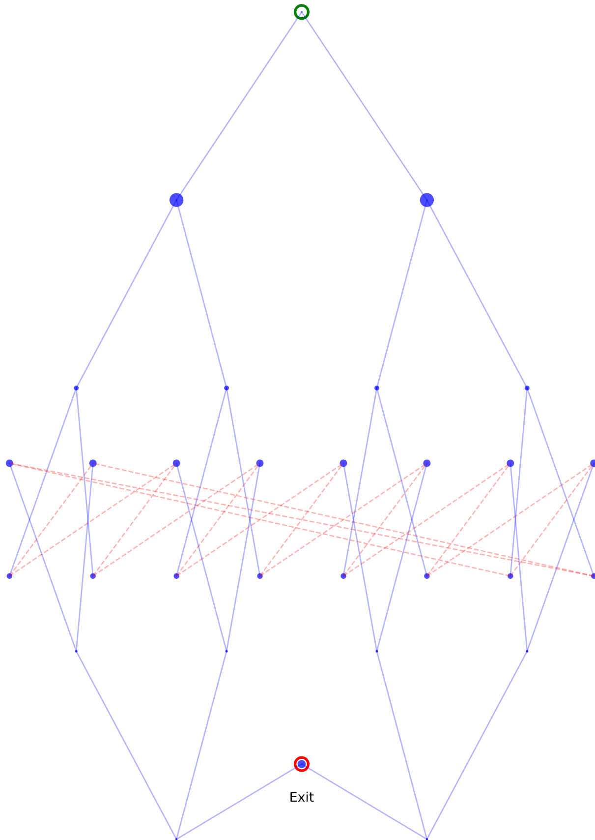
Quantum State Visualization at t = 8.25
