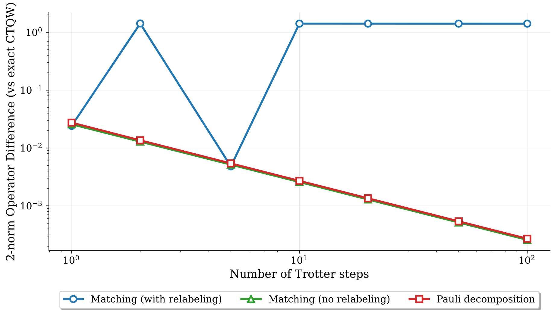
Circulant Graph C16(1,3,5) (4 qubits)
