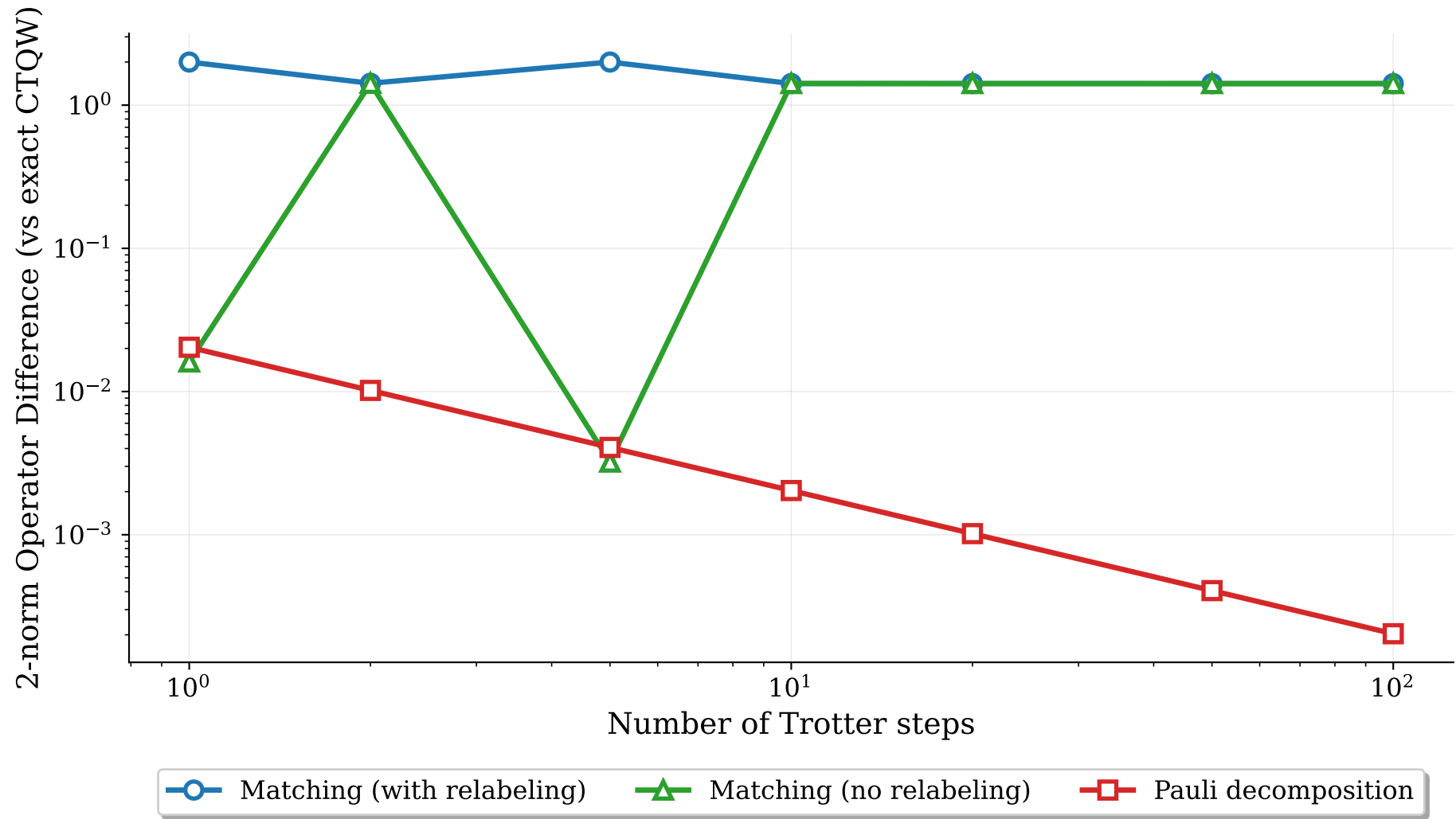
Circulant Graph C8(1,2) (3 qubits)
