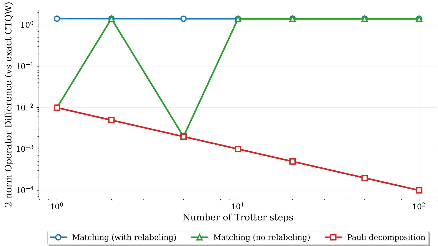
Complete Graph K4 - C2
