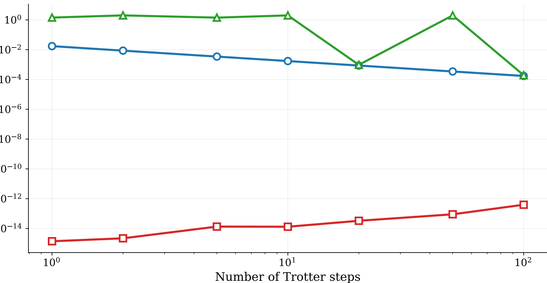
Dense Bipartite Graph (3 qubits)
