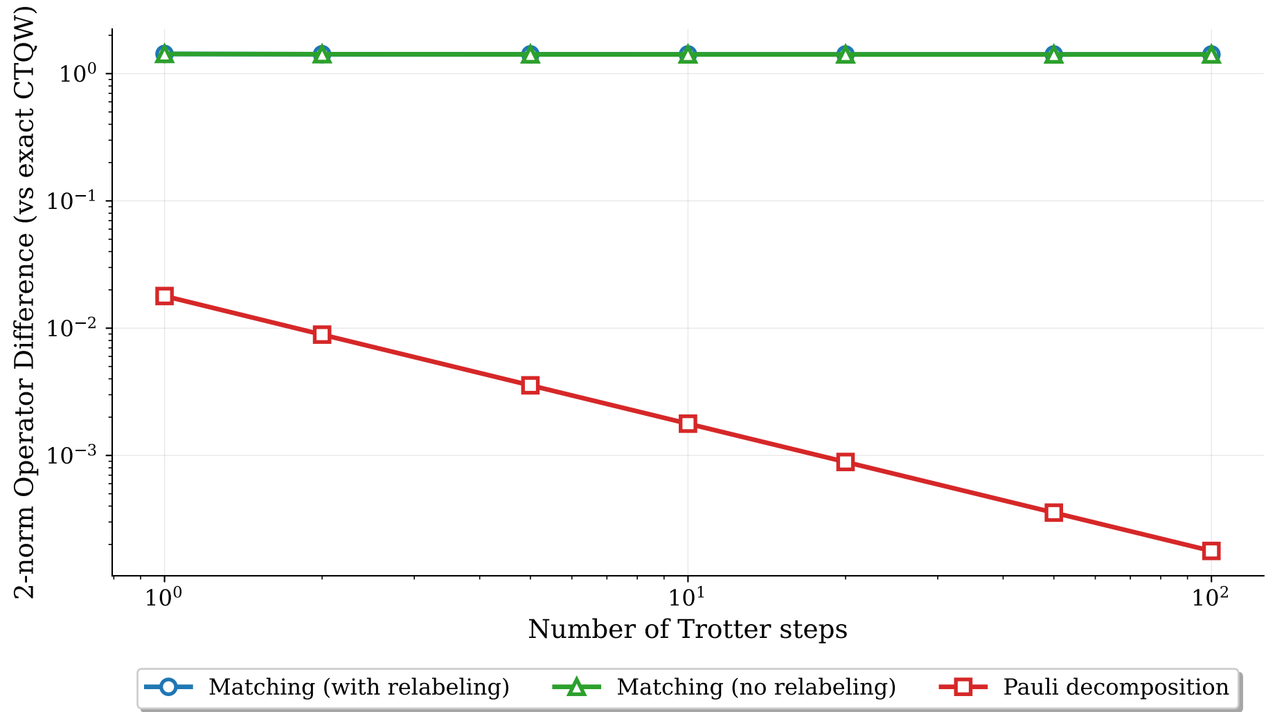
Dense Non-Bipartite Graph (3 qubits)
