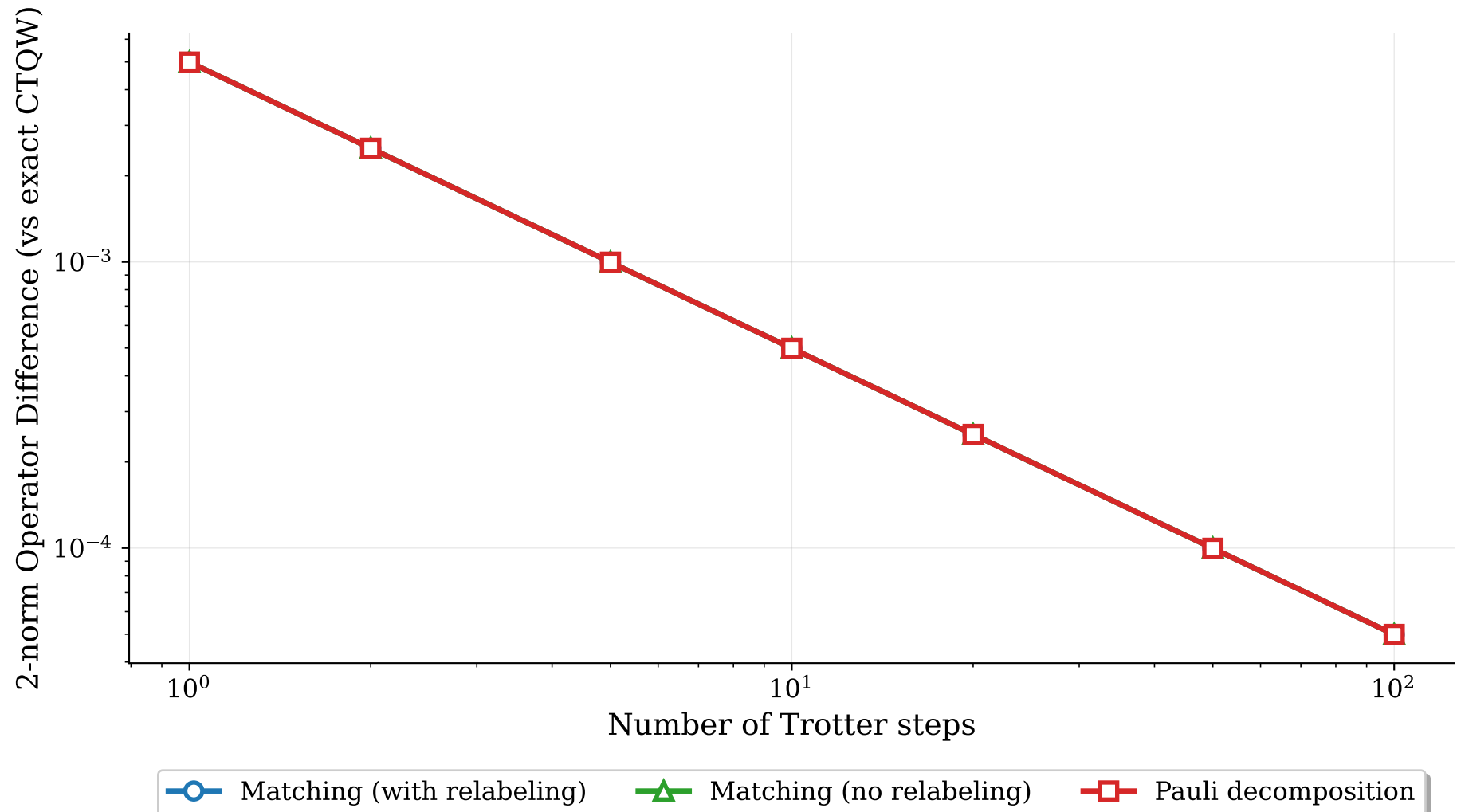
Path Graph P3
