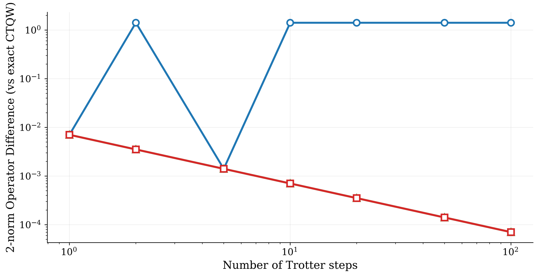
Sparse Non-Bipartite Graph (3 qubits)
