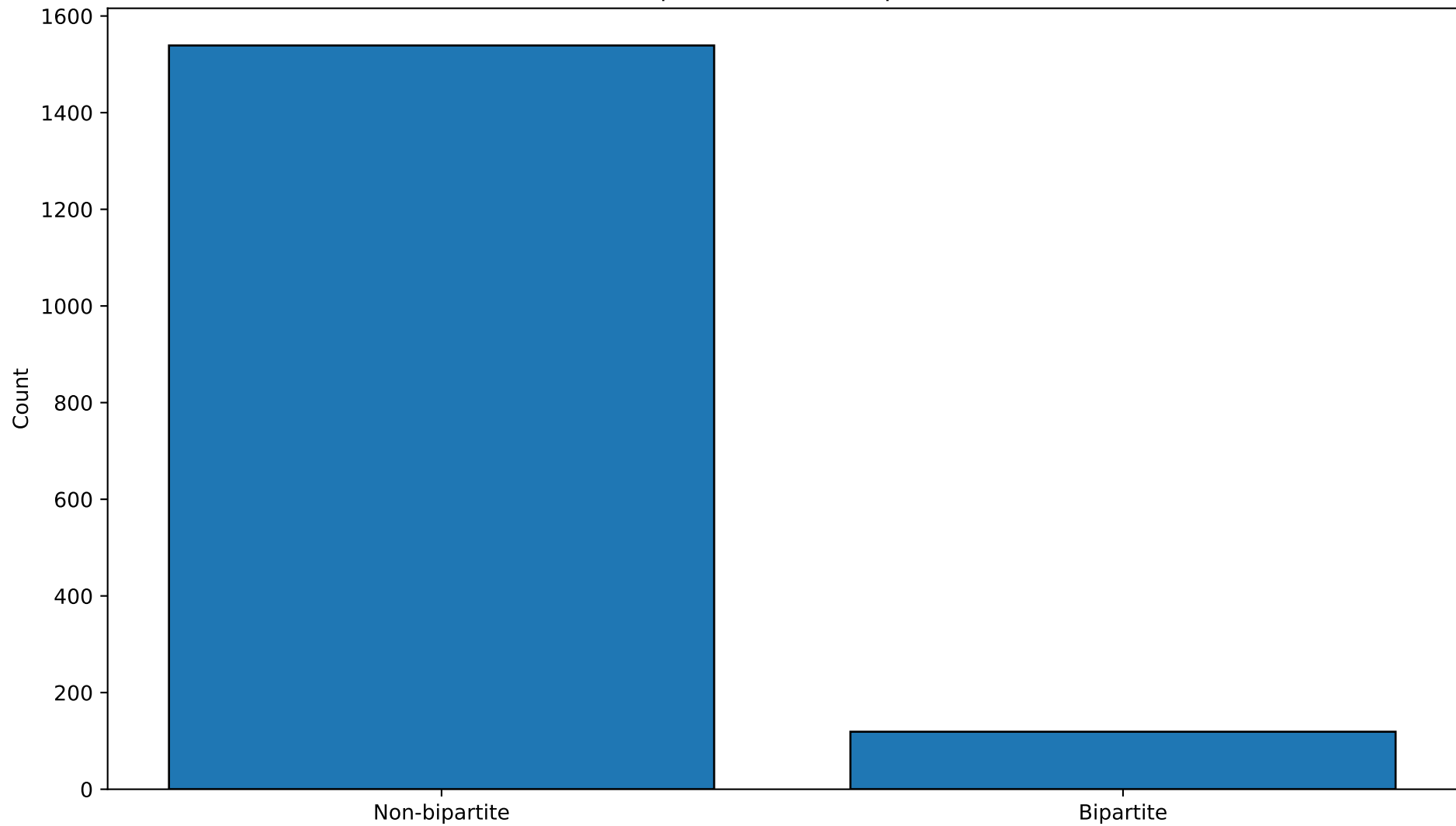
Bipartiteness of Graphs
