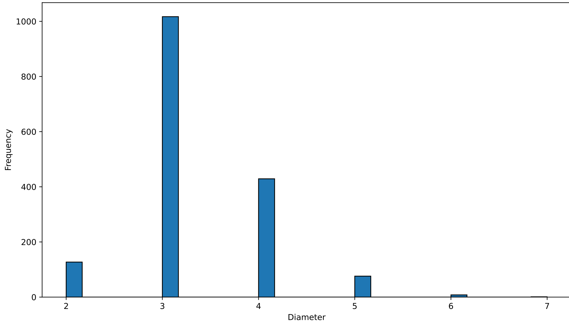
Distribution of Graph Diameters
