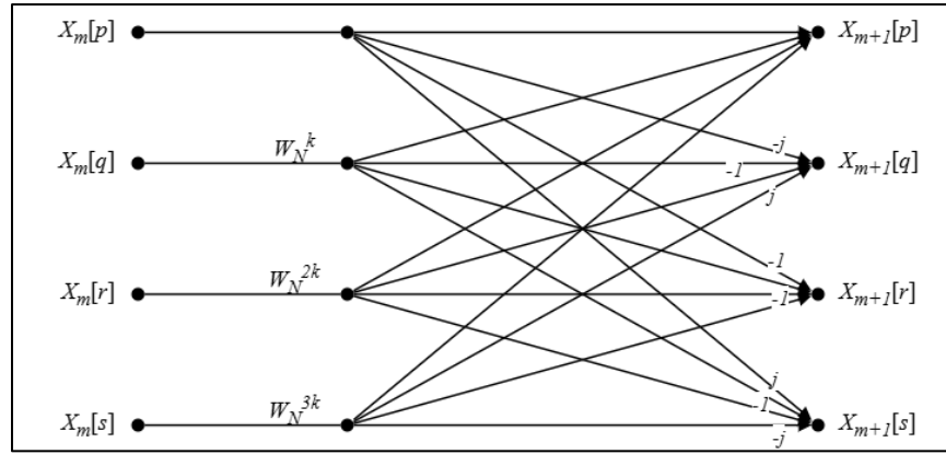
Figure 1.3: Radix-4 butterfly (adapted from [ch9][1])
