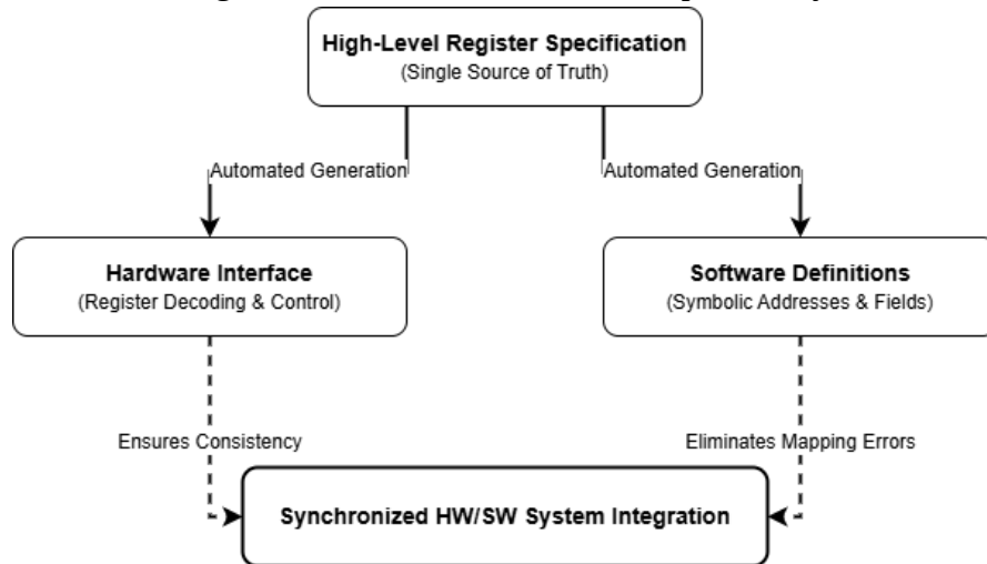
Figure 1.13: Register specification flow from description to generated hardware and software interfaces.
