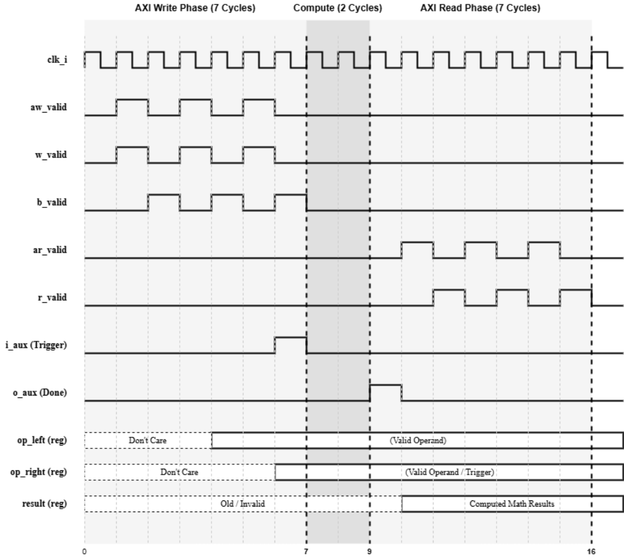
Figure 1.19: Timing diagram of the AXI-integrated butterfly accelerator
