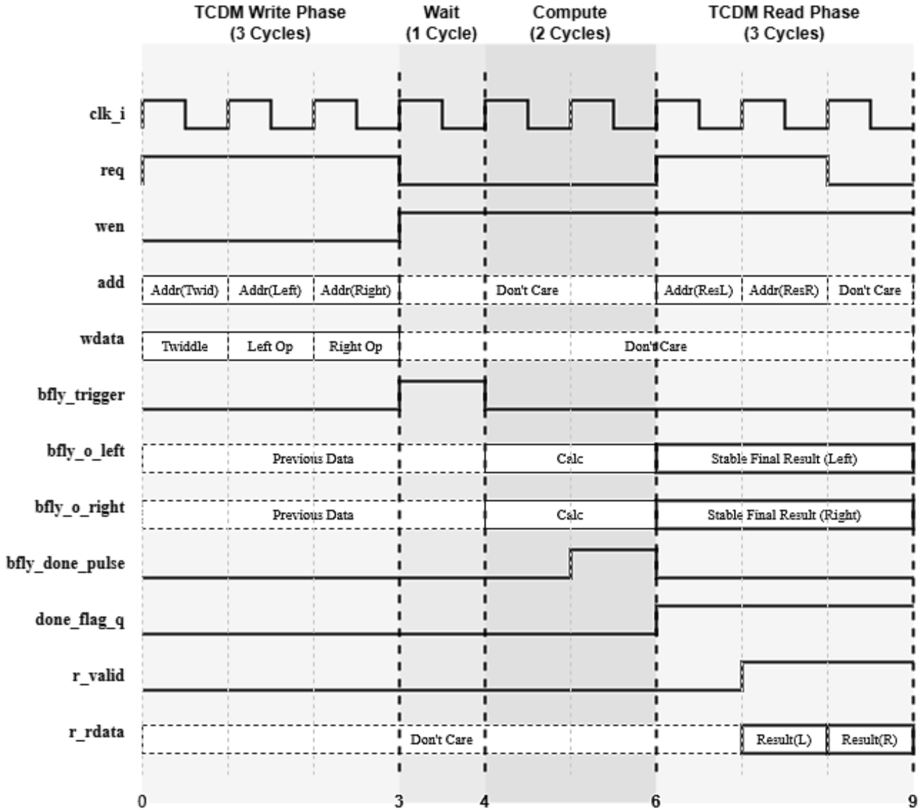
Figure 1.20: Timing diagram of the TCDM-integrated butterfly accelerator.
