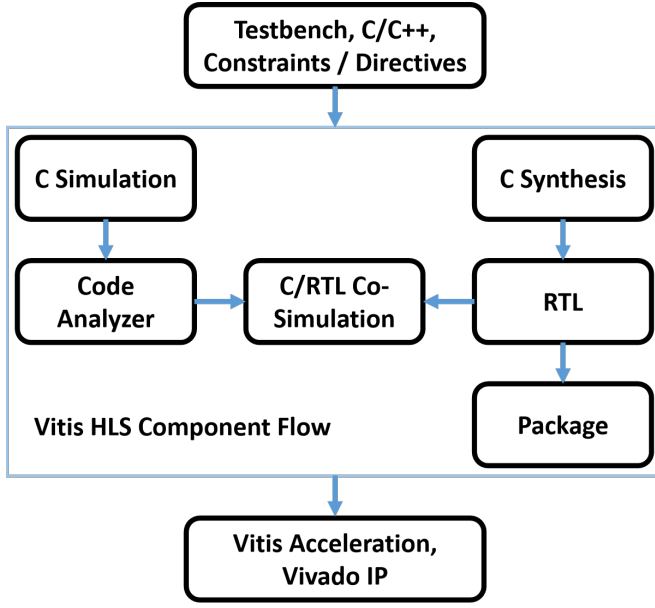
Fig. 2. Overview of the Tiny Transformer FPGA implementation workflow [15]
