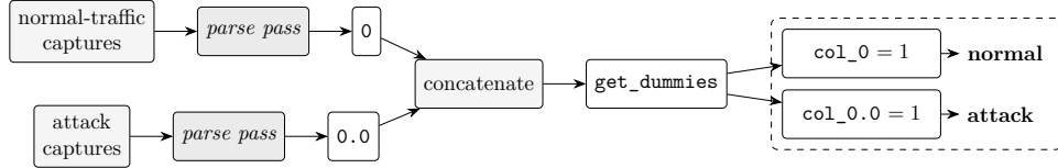
Figure 1: How file provenance becomes the label. The two captures were parsed in separate passes that serialise an absent field differently, and dummy encoding turns the two spellings into indicator columns. Since the files partition the classes, either column reproduces the label. No step involves network behaviour.
