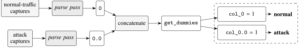
Fig. 1. How file provenance becomes the label. The two captures were parsed in separate passes that serialise an absent field differently, and dummy encoding turns the two spellings into indicator columns. Since the files partition the classes, either column reproduces the label. No step involves network behaviour.
