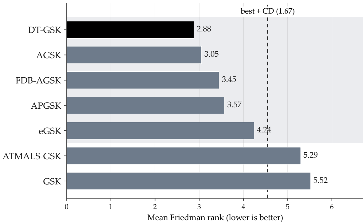
Nemenyi Critical Difference (CEC2017, D=10 , k=7 , N=29 , \alpha=0.05 )
