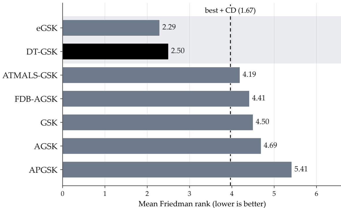
Nemenyi Critical Difference (CEC2017, D=30 , k=7 , N=29 , \alpha=0.05 )
