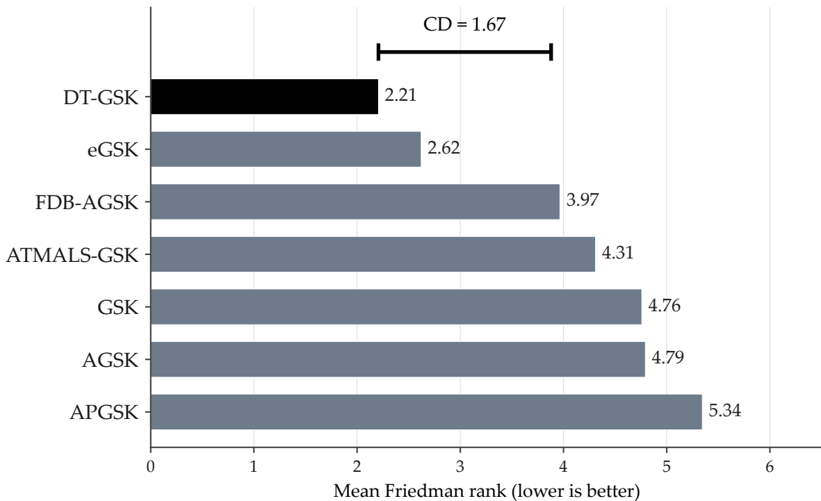
Nemenyi Critical Difference ( CEC2017, D=50, k=7, N=29, \alpha=0.05 )
