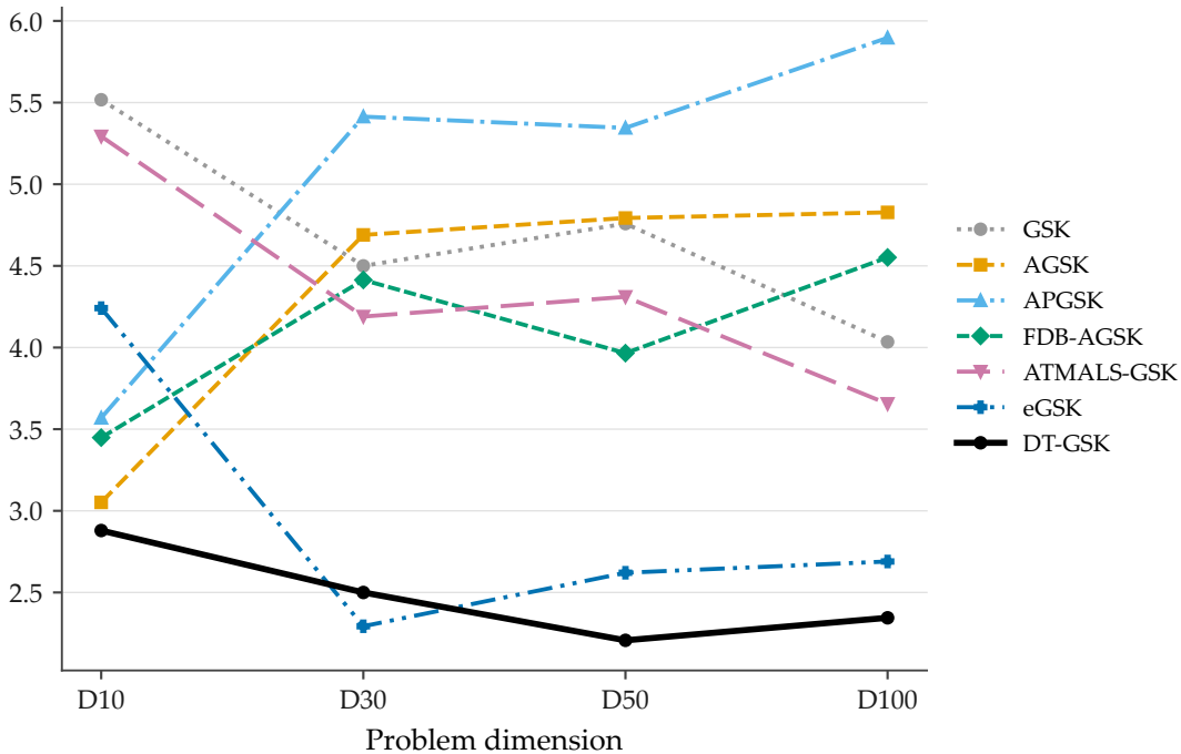
Mean Friedman rank (lower is better)
