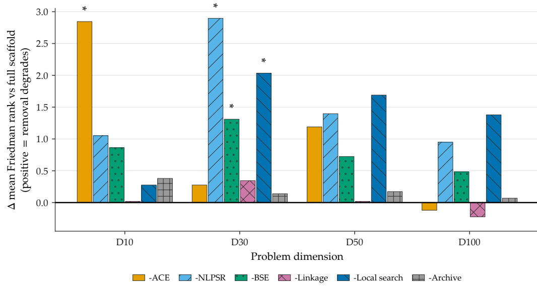
Figure B27. Conditional rank degradation from removing each scaffold component on CEC2017 (ISM off in every cell; 51 runs; 29 functions). Bars show the change in mean Friedman rank versus the full-scaffold baseline; positive means removing the component degrades rank. Colors follow the frozen per-cell palette; * marks Holm-significant contrasts within a dimension ( \alpha = 0.05 ). Each bar is a conditional remove-one contribution, not an independent causal effect, and bars are not averaged across dimensions.
