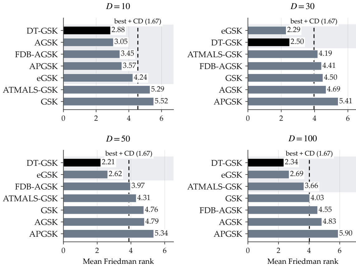
Figure 4. Critical-difference view of the CEC2017 GSK-family Friedman mean ranks (lower is better), one panel per dimension. Bars are mean ranks; the shaded rows are the cohort within one critical difference of the best rank, and the dashed line marks best rank + CD (CD = 1.67 for k = 7 , N = 29 , \alpha = 0.05 ). A bar crossing the line is Nemenyi-separated from the best; DT-GSK and eGSK fall inside one cohort at every dimension.
