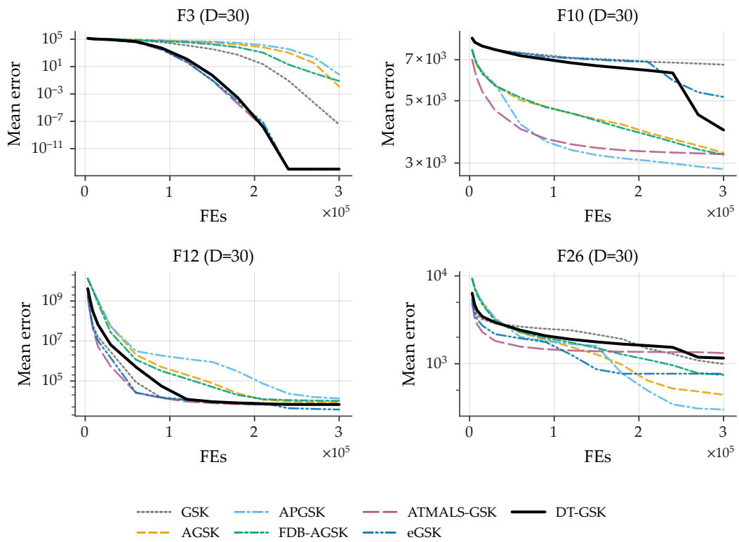
Figure 6. Family-overlay convergence on CEC2017 at D = 30 — DT-GSK’s known-weak tier, ranked second behind eGSK — for the four prespecified functions: F3 (unimodal; easy/strong), F10 (simple multimodal; hard/comparable), F12 (hybrid; hard/comparable), F26 (composition; hard/weak, the mandated unfavorable case). Shared basis as stated above; APGSK checkpoint evidence at D = 30 carries the per-run availability qualification of Section 4.1.
