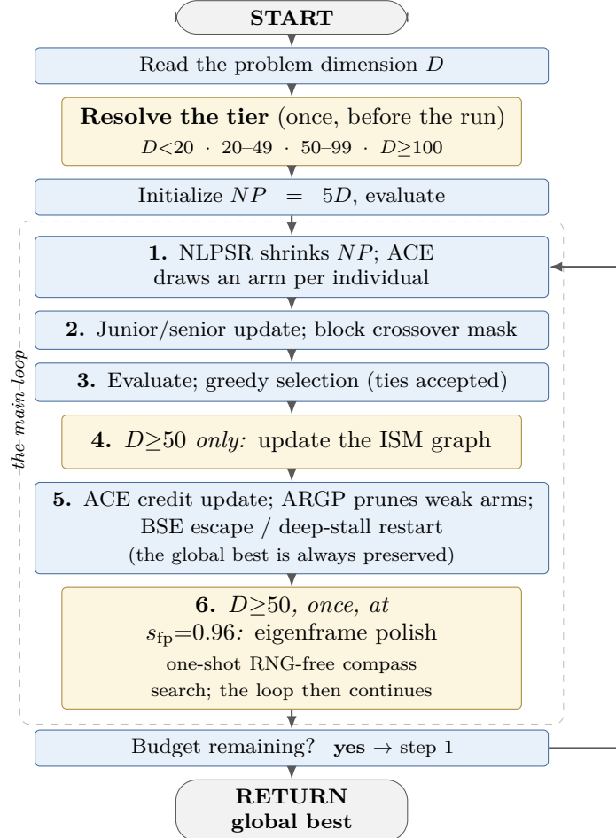
Figure 1. DT-GSK’s execution order. Gold marks the dimension-gated stages; the tier itself is fixed before the loop begins. The eigenframe polish is a one-shot stage inside the loop, not a closing step: it arms in the first generation that reaches s_{fp}=0.96 of the budget, is capped at 0.02 \text{ MaxFES} , and ordinary generations resume on the remainder.
