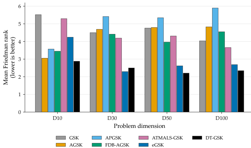
Figure 3. Friedman mean ranks per dimension (CEC2017, 29 functions, 51 runs), grouped by dimension in the fixed panel order; companion to Table 14. Lower is better. Rank-robustness and APGSK-gap qualifications as in Table 14.
